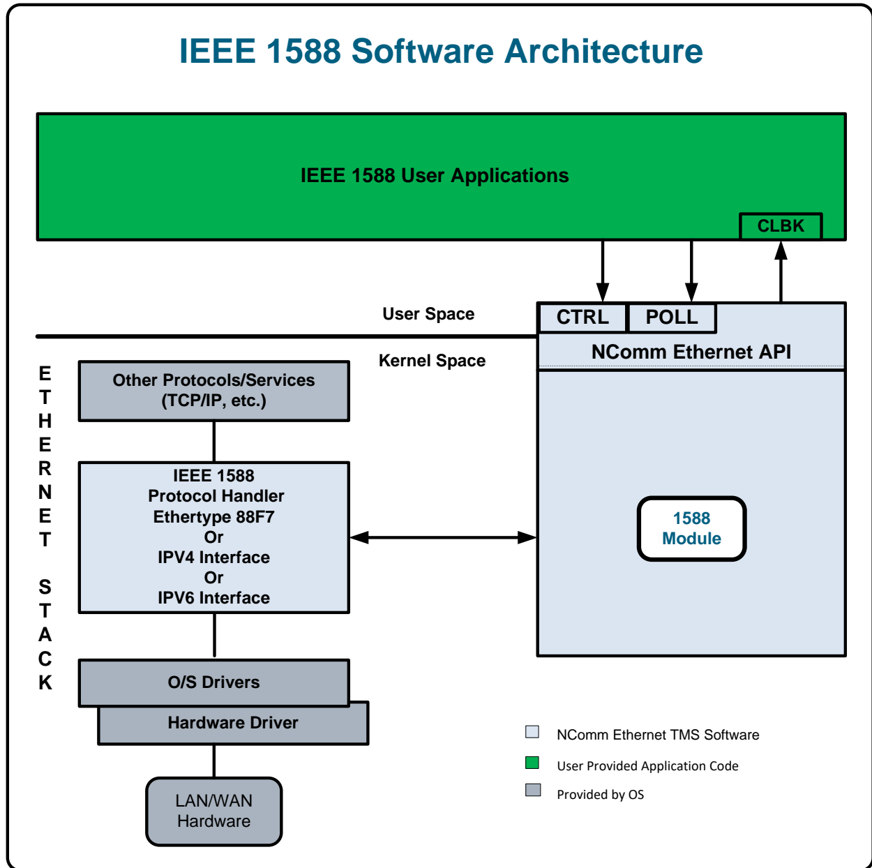
Driver and IEEE 1588 Software Architecture
